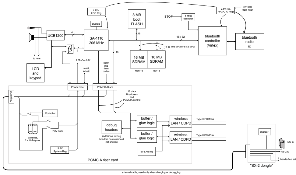
Personal Router Block Diagram, 1/16/00
